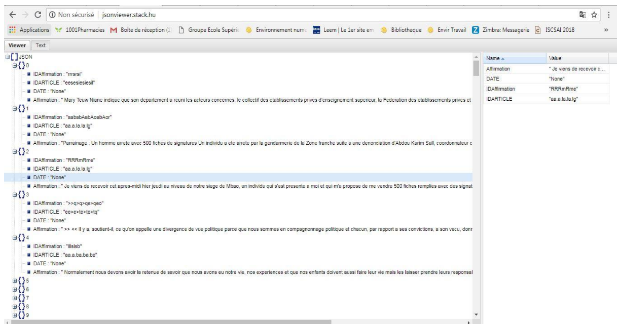
Figure 21. Affirmations. JSON
